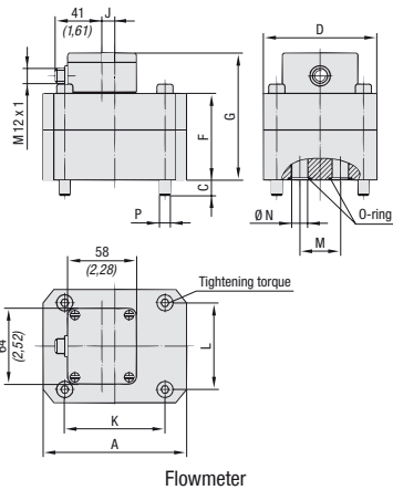
Flowmeter
