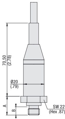
Flying Leads
